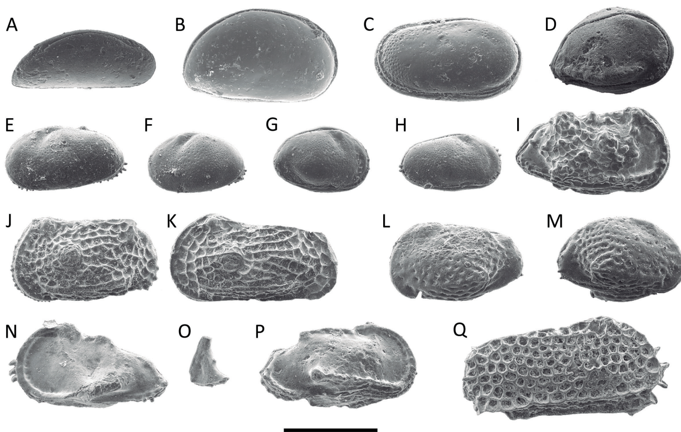
Figure 9. Ostracod carapaces from interval 11 of La Dehesa locality (late Albian–early Cenomanian; Esterciel, Aragón, Spain). A , Paracypris sp., MPZ 2024/28; B , Asciocythere aff. compressa , MPZ 2024/29; C , Cytherella sp., MPZ 2024/30; D , Schuleridea alata , MPZ 2024/46; E–F , Schuleridea jonesiana , male and female carapace respectively, MPZ 2024/41 and MPZ 2024/43; G–H , Schuleridea sp., male and female carapace respectively, MPZ 2024/44 and MPZ 2024/42; I , Cythereis ( Rehacythereis ) cf. pseudobartensteini , MPZ 2024/33; J–K , Oertiella sp., male and female carapace respectively, MPZ 2024/39 and MPZ 2024/36; L–M , Cytheropteron sp., male and female carapace respectively, MPZ 2024/38 and MPZ 2024/40; N–O , Pterygocythereis cf. robusta , fragment in O was broken during the preparation of the SEM stub, MPZ 2024/34; P , Pterygocythereis gr. pulvinata , MPZ 2024/35; Q , Platycythereis degenerata , MPZ 2024/37. All at the same scale; scale bar = 0.5 mm.
